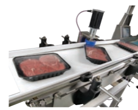
Pack Turner Turns packs to wide edge leading for correct presentation to the labeller.
