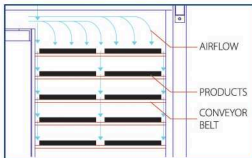
Vertical airflow pushes product into the Mesh belt
